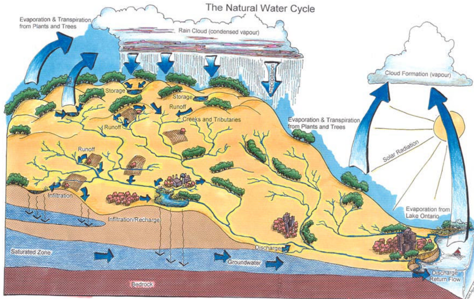
FIGURE 2-1: THE NATURAL WATER CYCLE
